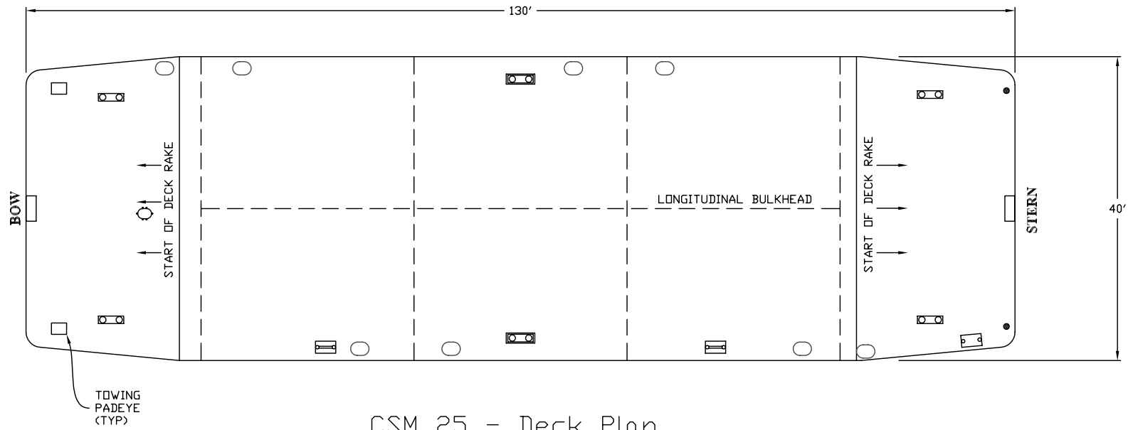
CSM 25 - Deck Plan
